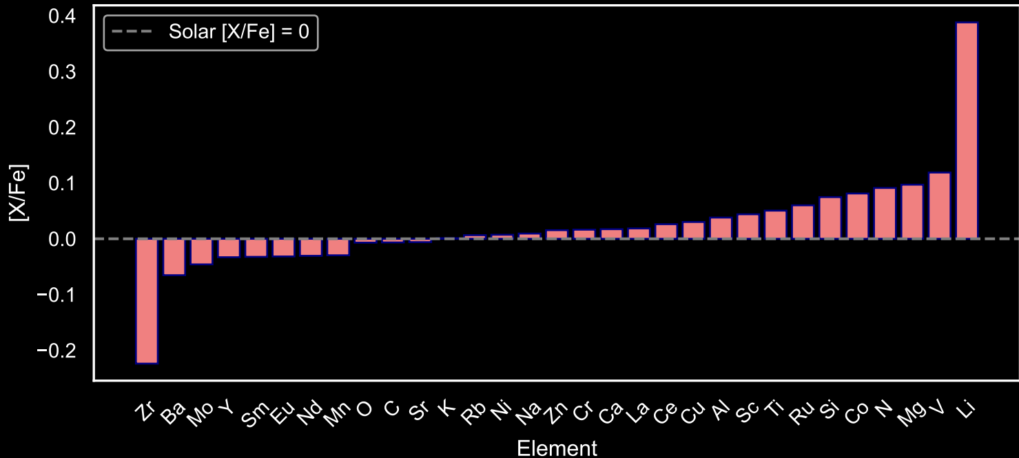
Abundance Pattern for GALAH Main Sequence Stars: Star Field [49] (N=141)
