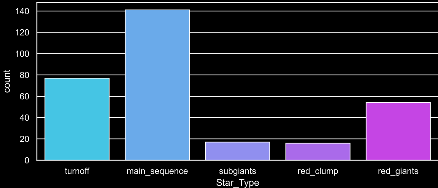
Field [49] Count plot of Star Type
