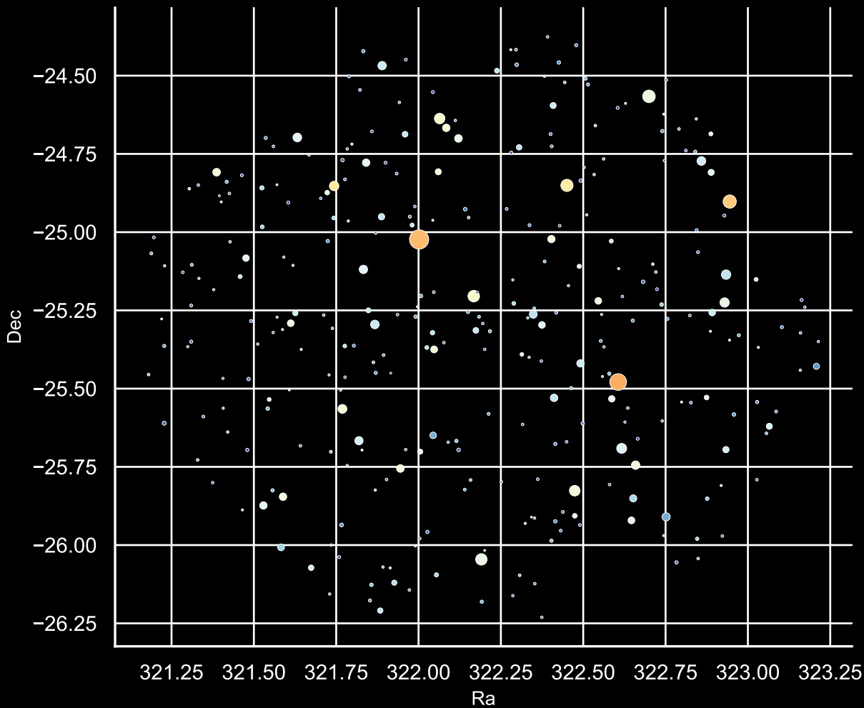
Field [49] Ra [322.17] Dec [-25.29] Stars: 305
