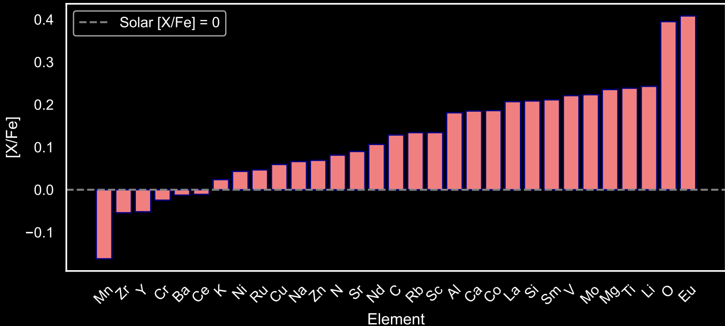
Abundance Pattern for GALAH Red Giants: Star Field [49] (N=70)
