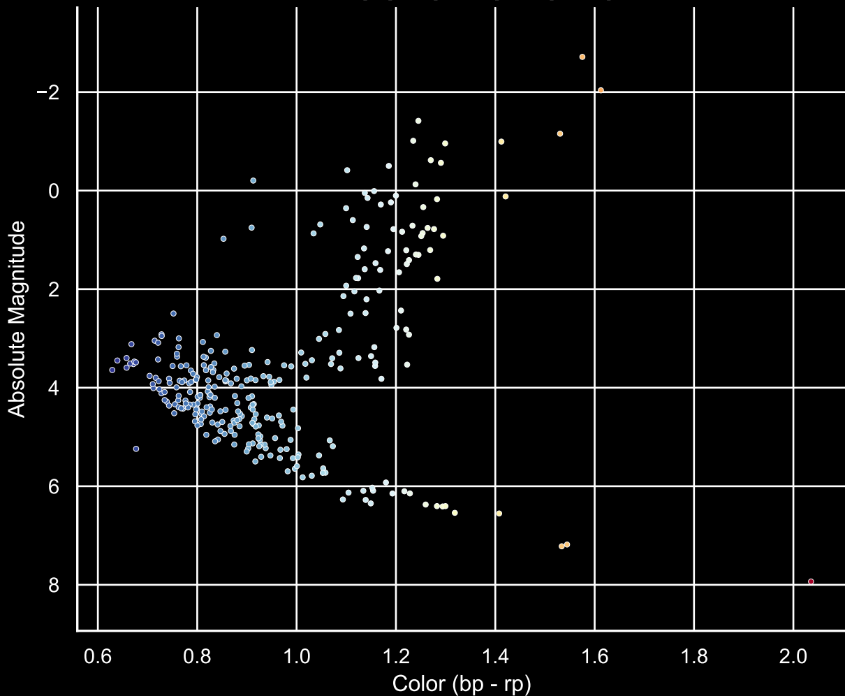
GALAH Hertzsprung-Russel Diagram Field [49] Ra [322.17] Dec [-25.29]
