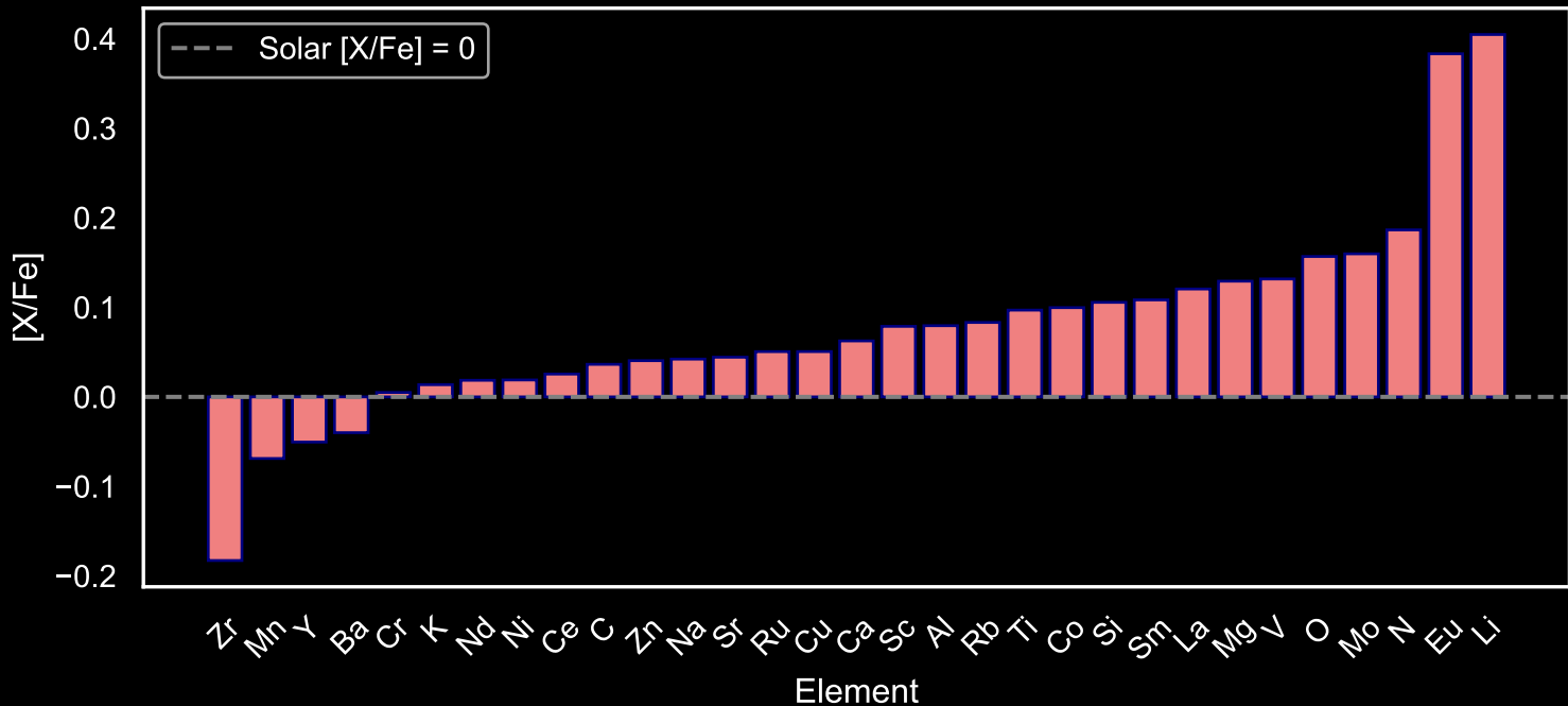
Abundance Pattern for GALAH Star Field [49] (N=305)
